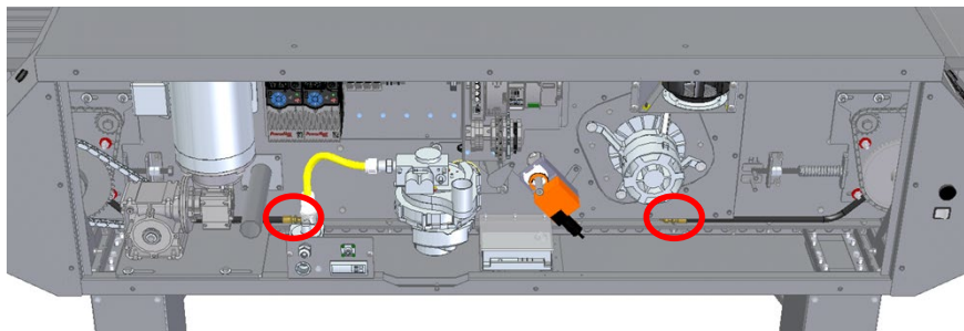
Remove the electrical panel
